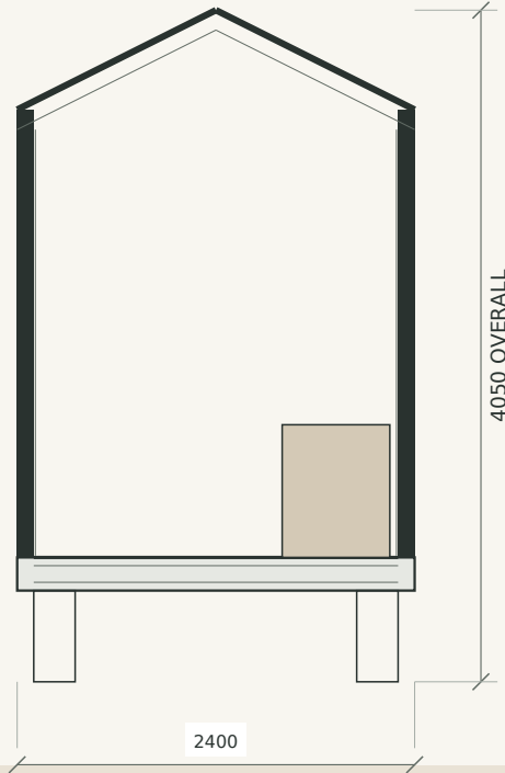
SECTION A-A / THROUGH LIVING 1:50
